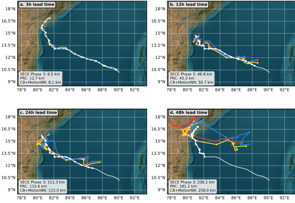
Figure 4: Cyclone Laila (2010) on held-out seed 0 (05_case_study_trajectories.csv). Four panels show 3, 12, 24, and 48 h lead times. White solid: storm centre at each origin; white dashed with markers: verified IBTrACS position at that lead. Coloured tracks are SECE Phase 3, PRC, and CB+MotionNN direct endpoints from each origin (not a rolled-out trajectory). Median great-circle errors in km appear in each panel.
